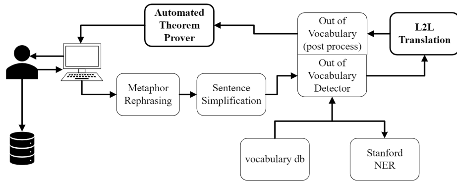
Fig. 1. Language to logic architecture
